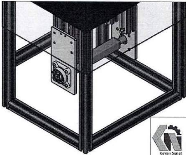
DETAIL E SCALE 1 : 7
